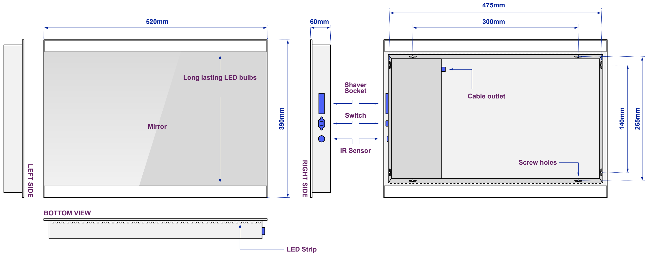
View of Back plate
