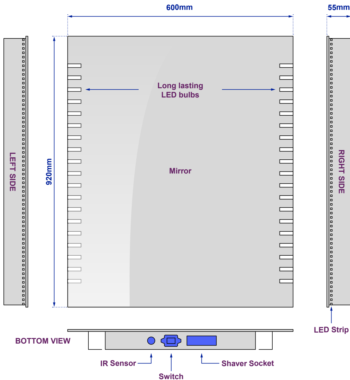
Views of complete assembly
