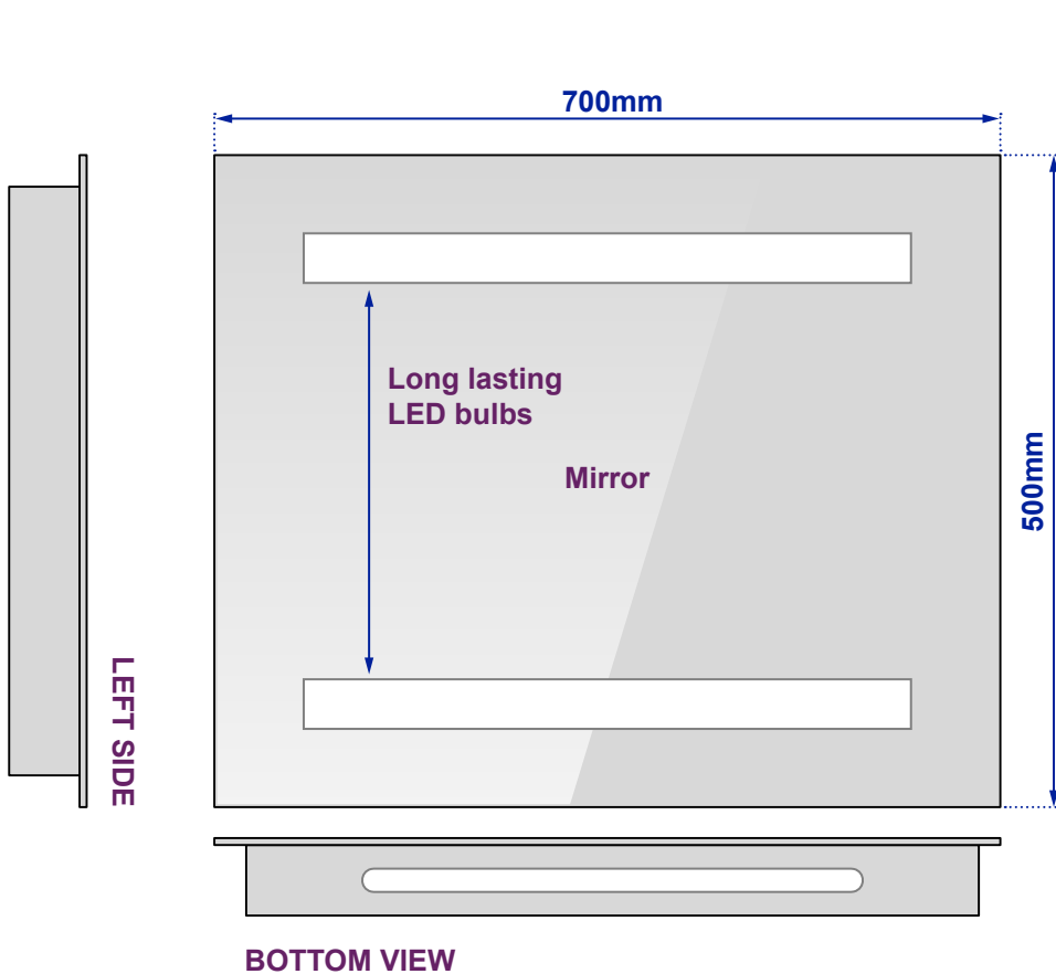
Views of complete assembly - With Mirror
