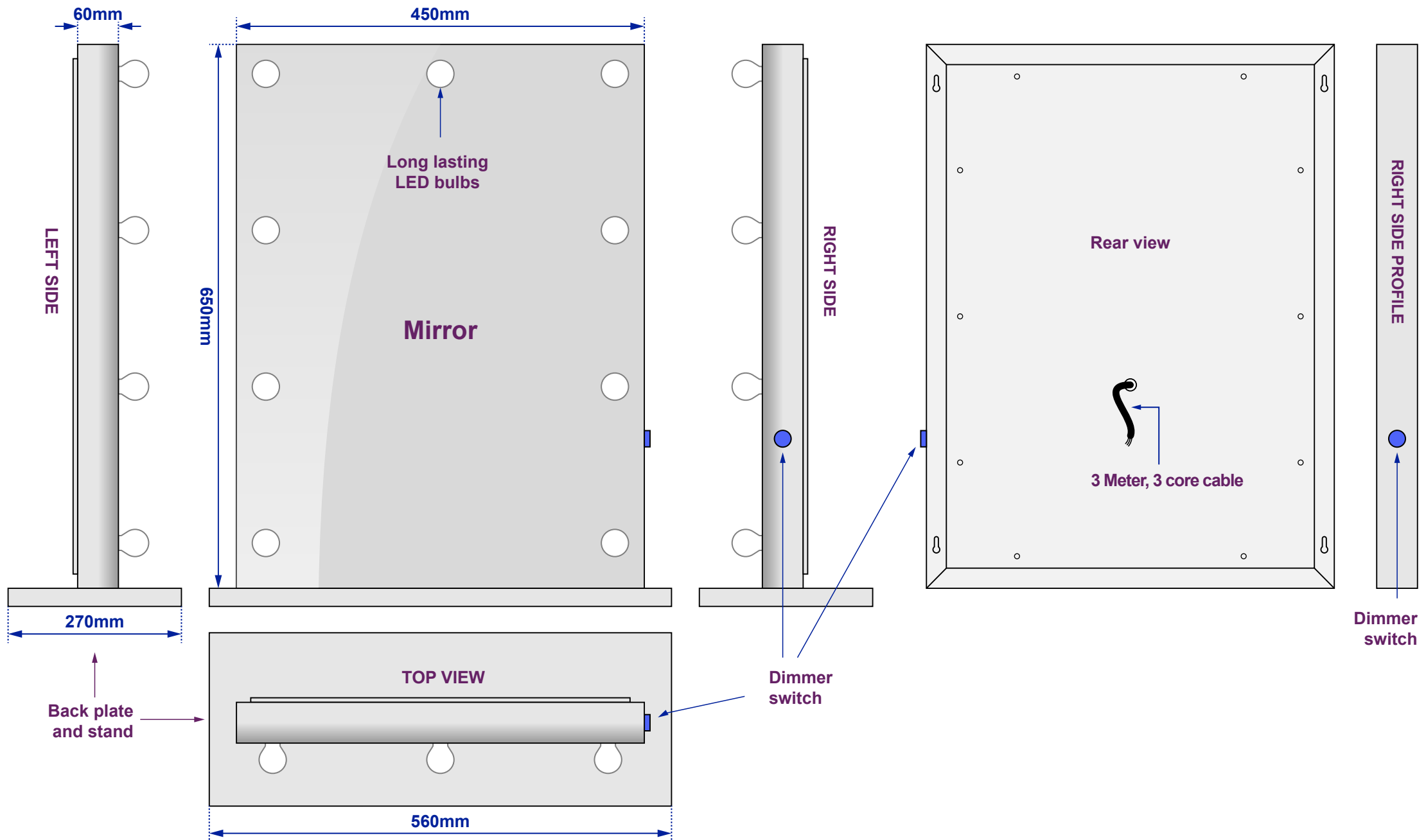
Views of completed stand assembly - with bulbs in place
