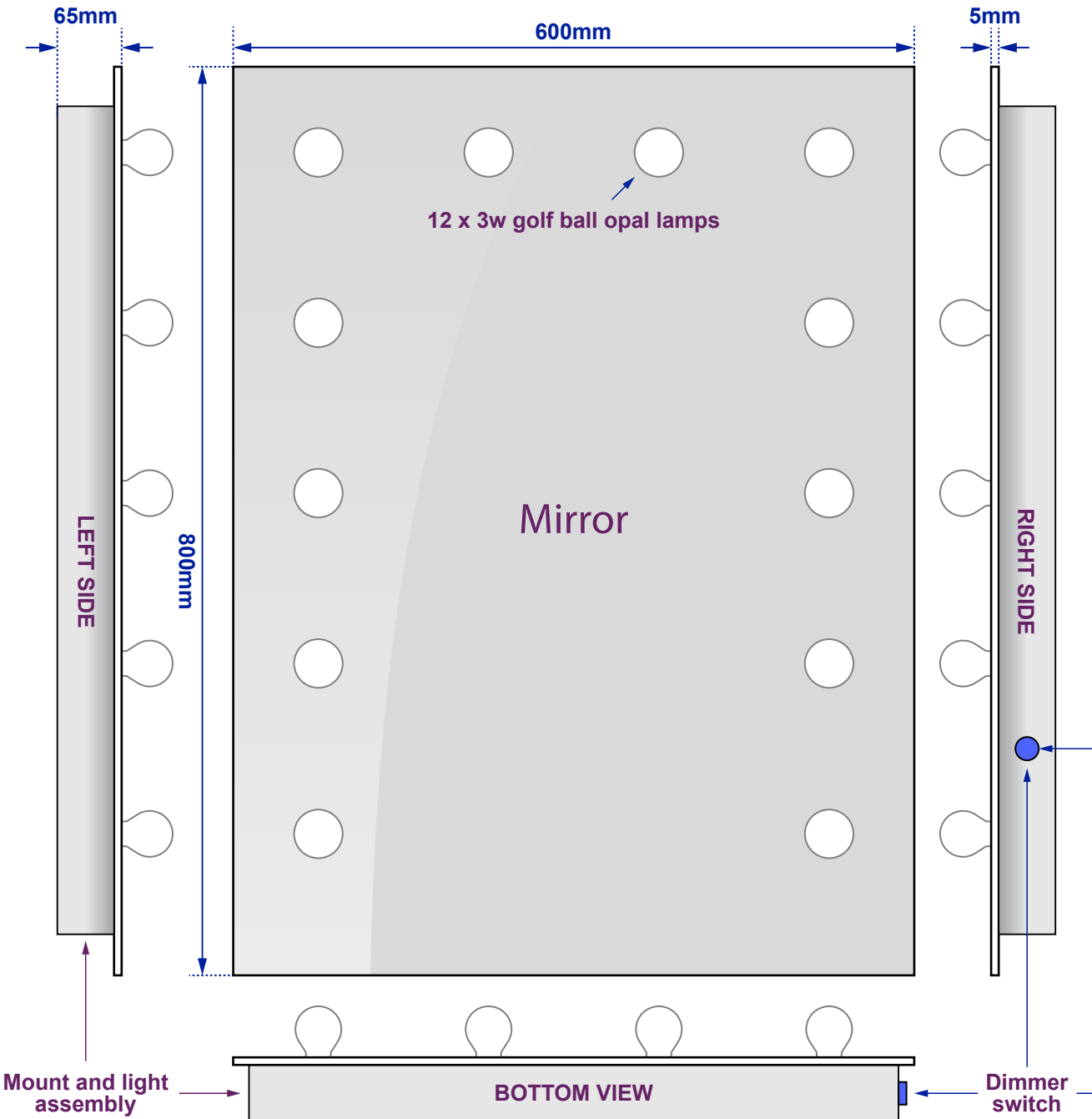
Views of complete assembly - With Mirror
